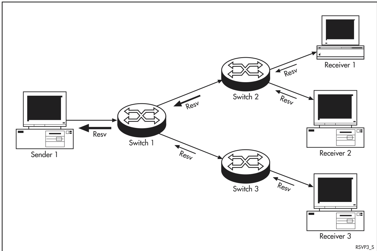
Figure 37-3: RSVP Resv messages travel from the receiver to the sender
