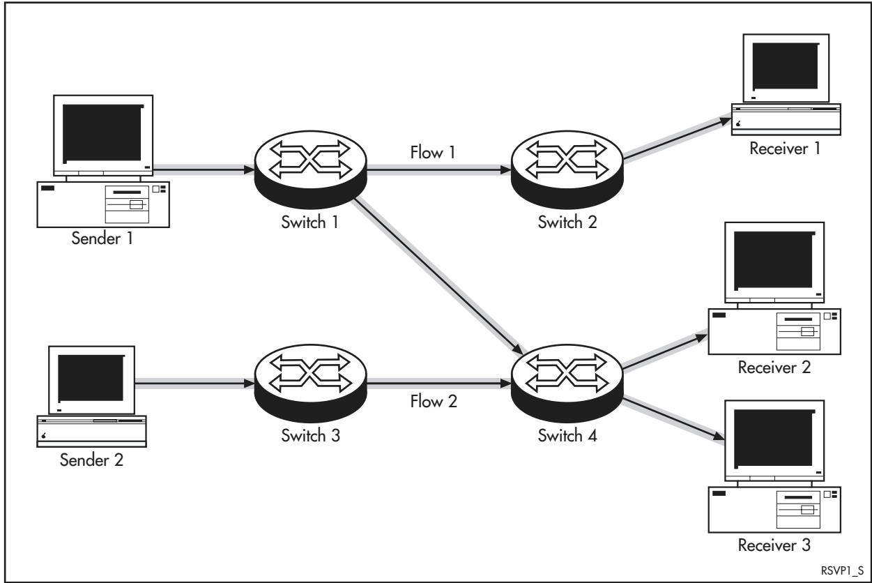
Figure 37-1: RSVP sessions with multicast receiver addresses
