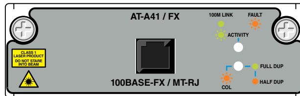
Figure 7: AT-A41-FX (MT-RJ) Uplink module.
