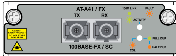
Figure 6: AT-A41-FX (SC) Uplink module.
